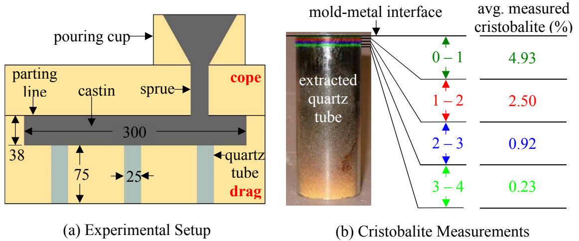
Figure 5.3 Using the experimental setup depicted in (a), minimal amounts of cristobalite were measured from the silica sand contained the quartz tubes (b), which were extracted after the casting cooled to room temperature. All dimensions in mm.
