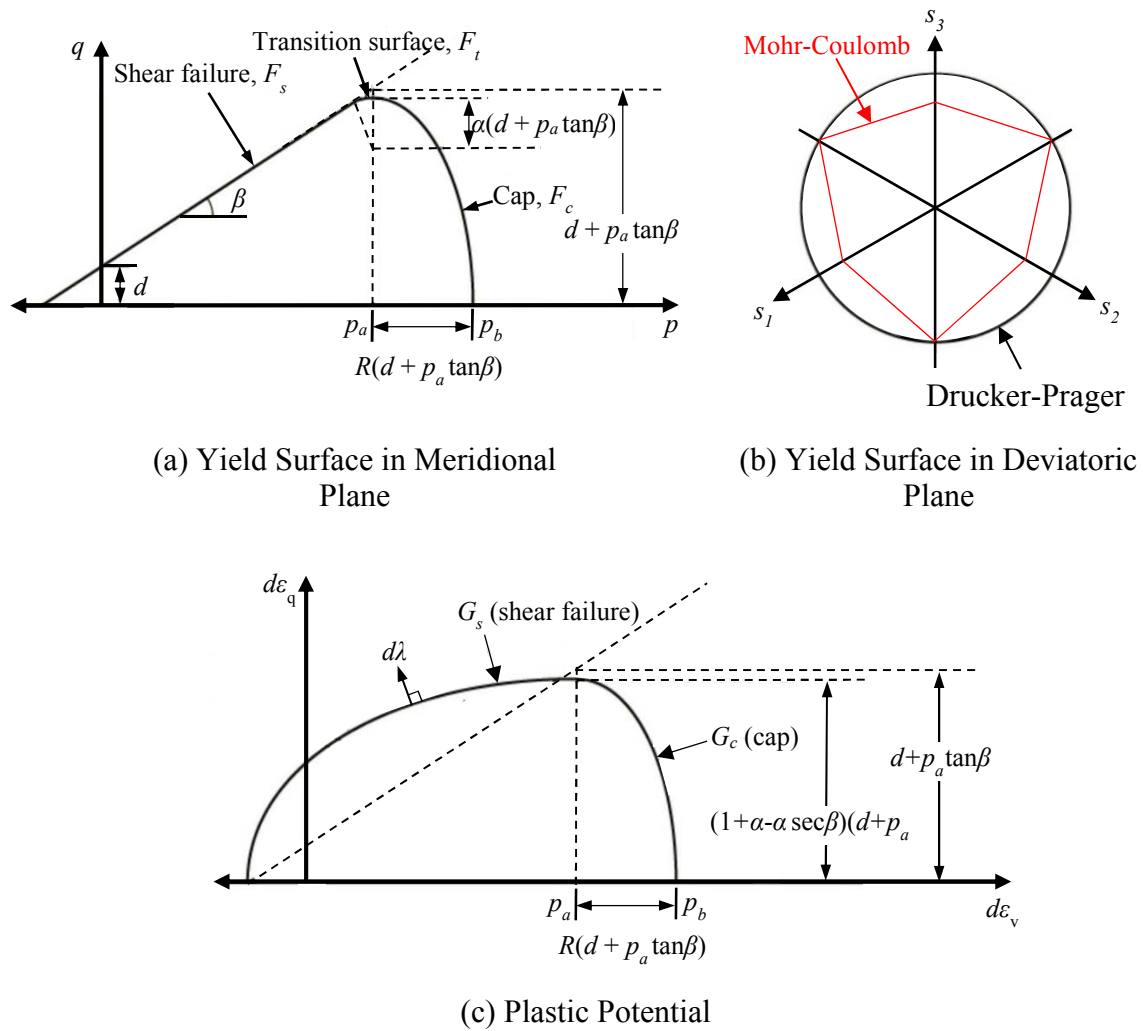
Figure 4.4. The Drucker Prager Cap yield surface in the meridional (a) and deviatoric (b) planes. The plastic potential (c) uses associated and non-associated flow rules for the cap and failure surfaces, respectively.
