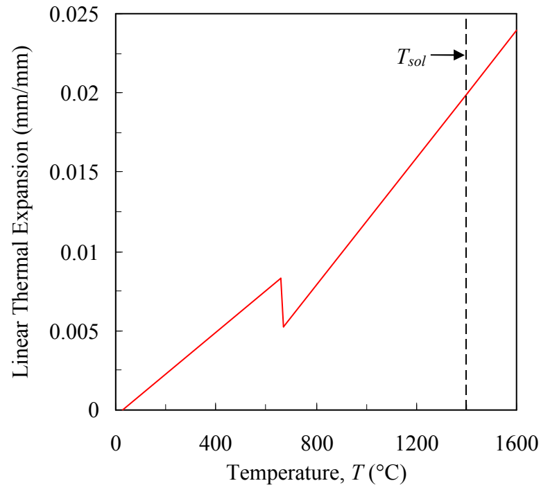
Figure 4.3. Linear thermal expansion for the steel.
