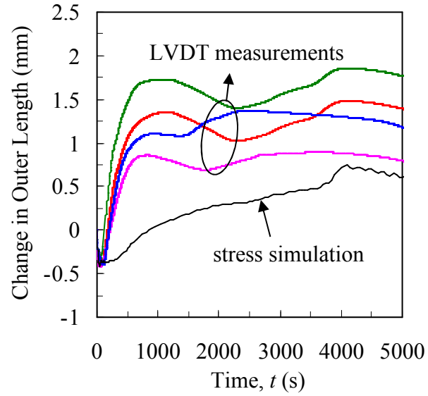
Figure 5.13 Comparison between measured and predicted changes in inner outer length using estimated bonded sand properties.
